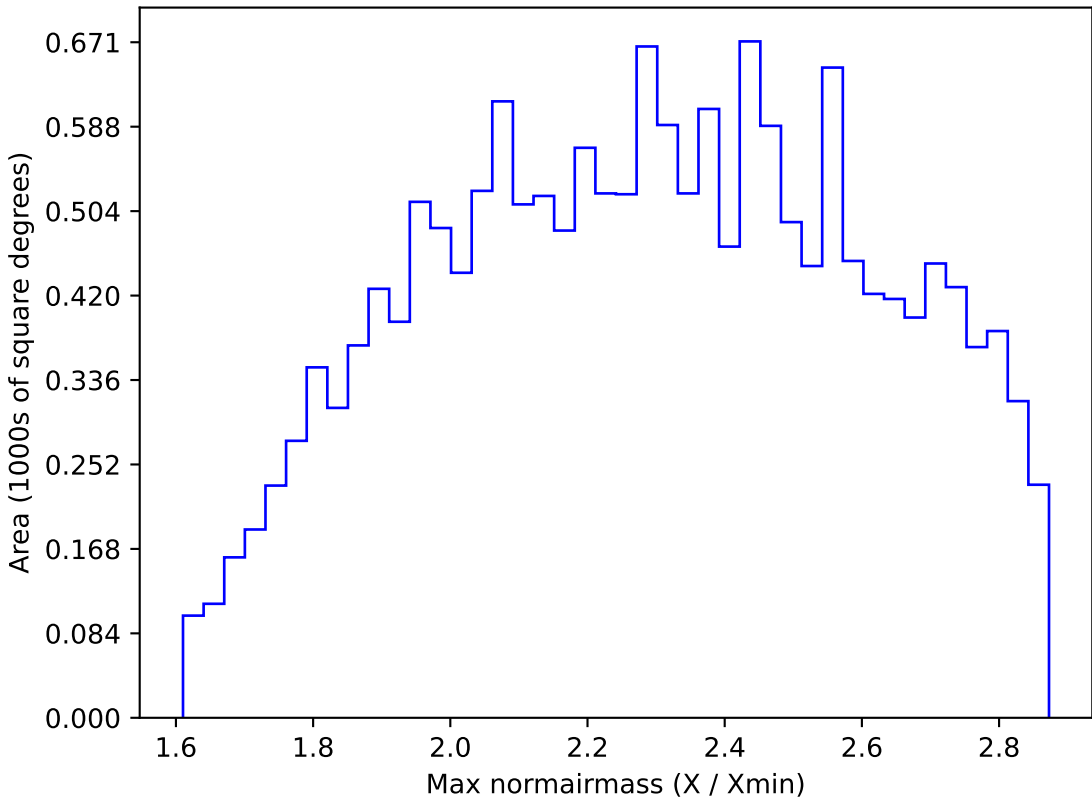
too_elab_r64_d3_ugrizy_v3.4_10yrs WFD z band: Max normairmass
