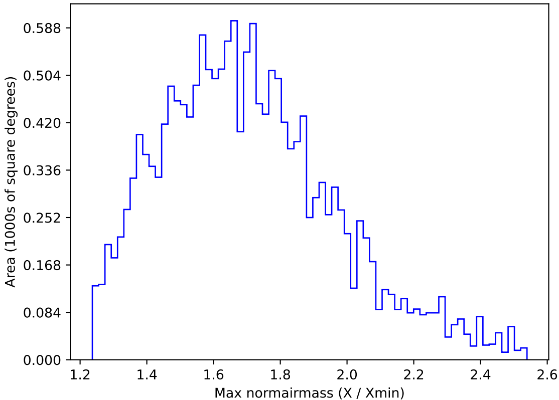
too_elab_r64_d3_ugrizy_v3.4_10yrs WFD u band: Max normairmass
