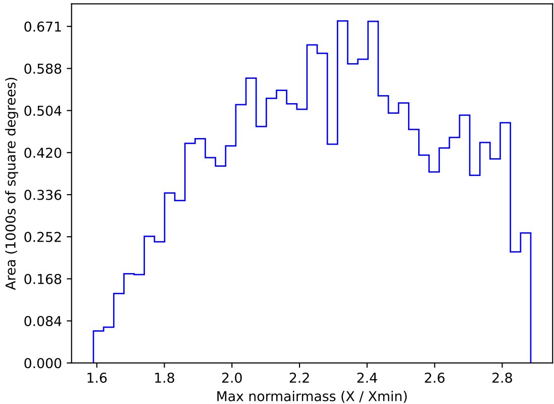
too_elab_r64_d3_ugrizy_v3.4_10yrs WFD i band: Max normairmass
