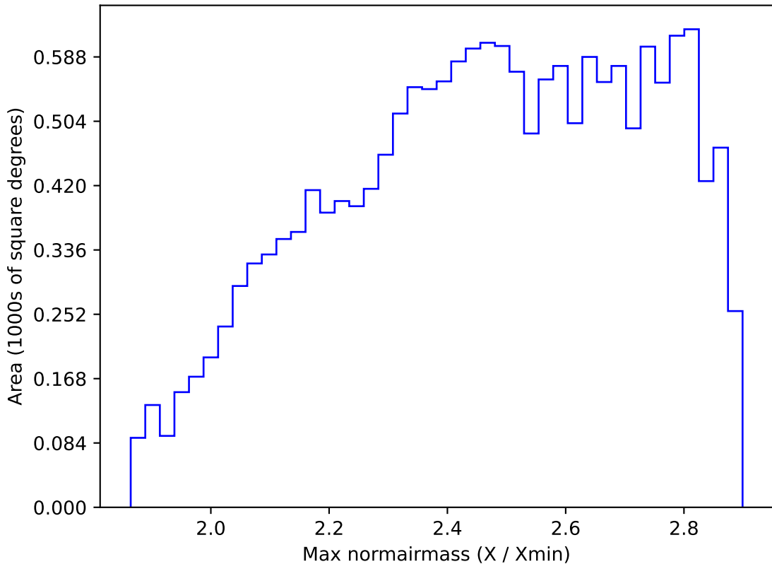
too_elab_r64_d3_ugrizy_v3.4_10yrs WFD all bands: Max normairmass
