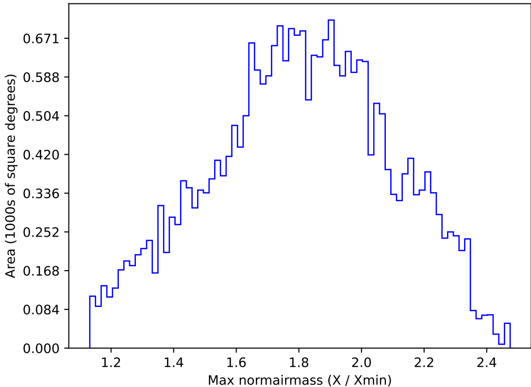
too_elab_r64_d3_ugrizy_v3.4_10yrs All sky g band: Max normairmass
