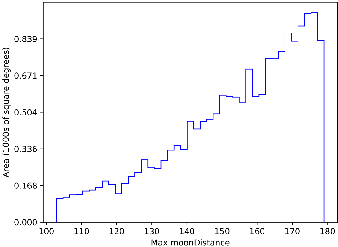
too_elab_r64_d3_ugrizy_v3.4_10yrs WFD z band: Max moonDistance
