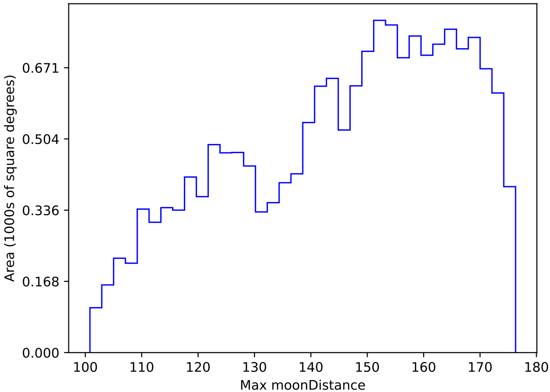
too_elab_r64_d3_ugrizy_v3.4_10yrs WFD y band: Max moonDistance
