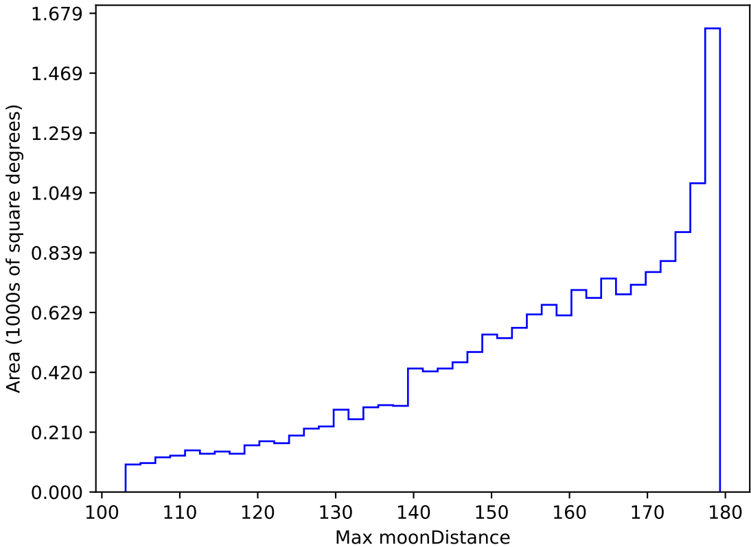
too_elab_r64_d3_ugrizy_v3.4_10yrs WFD r band: Max moonDistance
