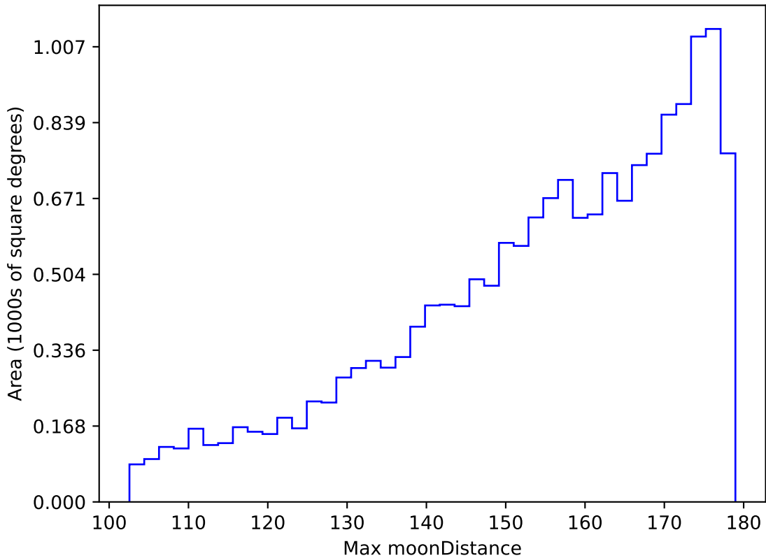
too_elab_r64_d3_ugrizy_v3.4_10yrs WFD g band: Max moonDistance
