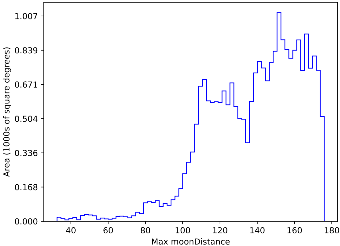
too_elab_r64_d3_ugrizy_v3.4_10yrs All sky y band: Max moonDistance
