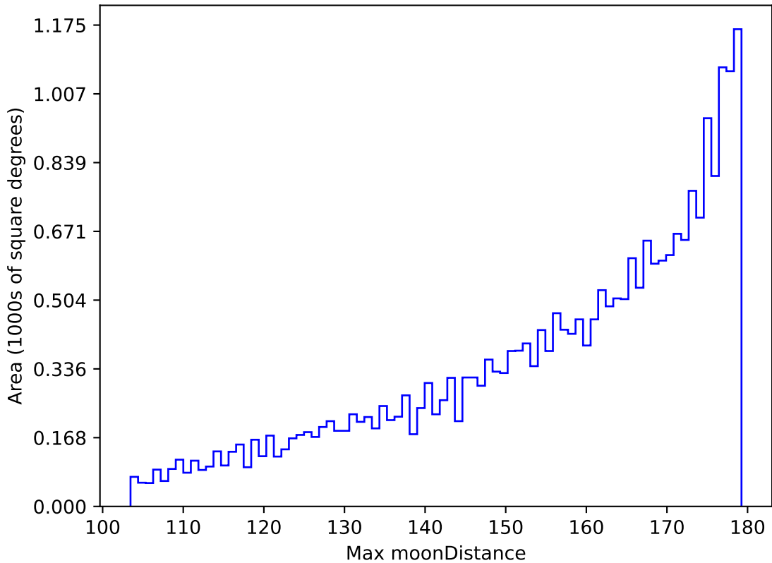
too_elab_r64_d3_ugrizy_v3.4_10yrs All sky r band: Max moonDistance
