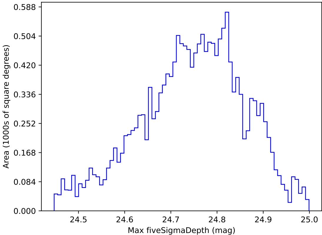
too_elab_r64_d3_ugrizy_v3.4_10yrs WFD r band: Max fiveSigmaDepth
