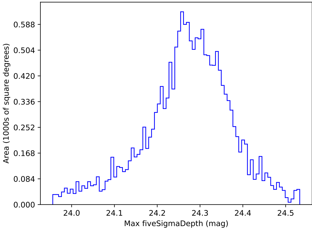
too_elab_r64_d3_ugrizy_v3.4_10yrs WFD i band: Max fiveSigmaDepth
