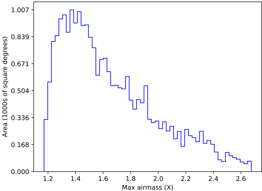
too_elab_r64_d3_ugrizy_v3.4_10yrs Yr 1 y band: Max airmass
