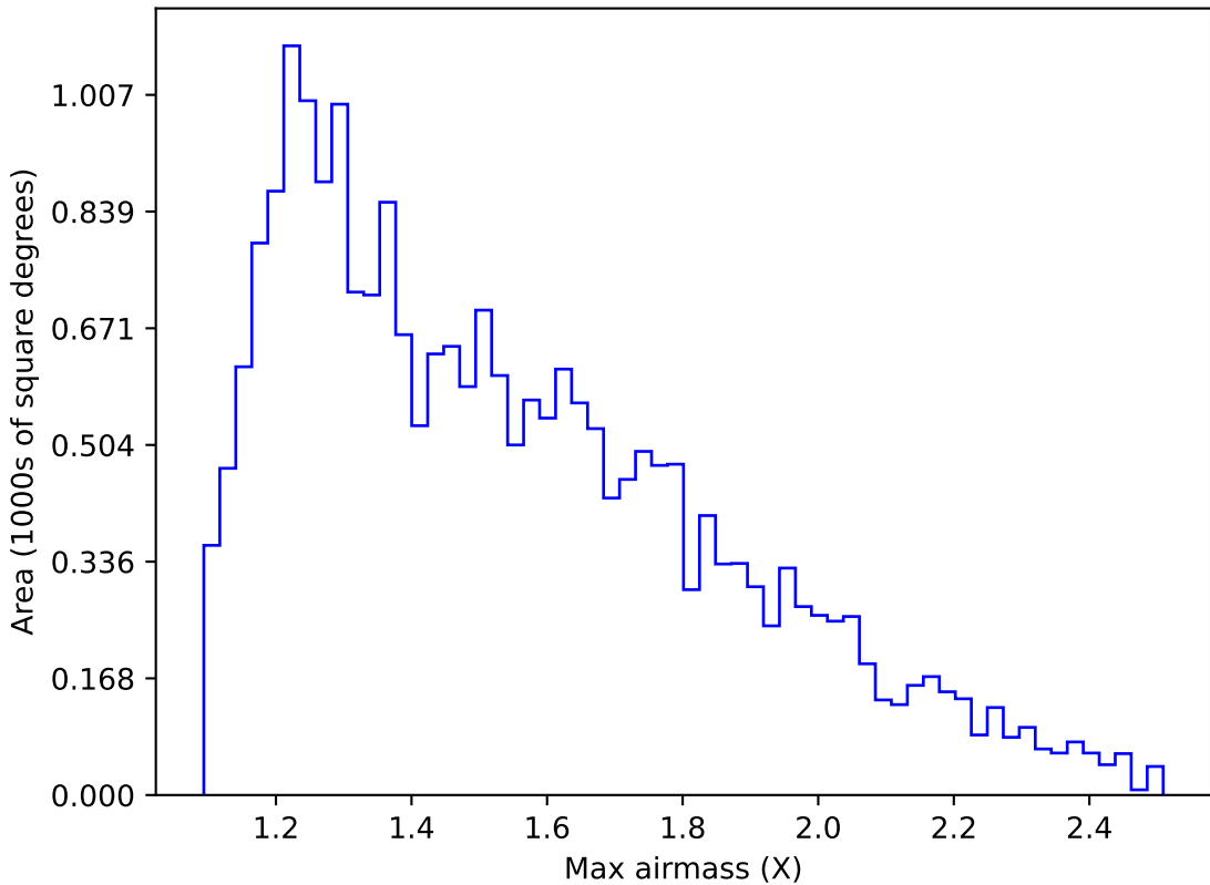
too_elab_r64_d3_ugrizy_v3.4_10yrs Yr 1 u band: Max airmass
