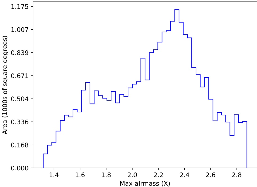
too_elab_r64_d3_ugrizy_v3.4_10yrs Yr 1 all bands: Max airmass
