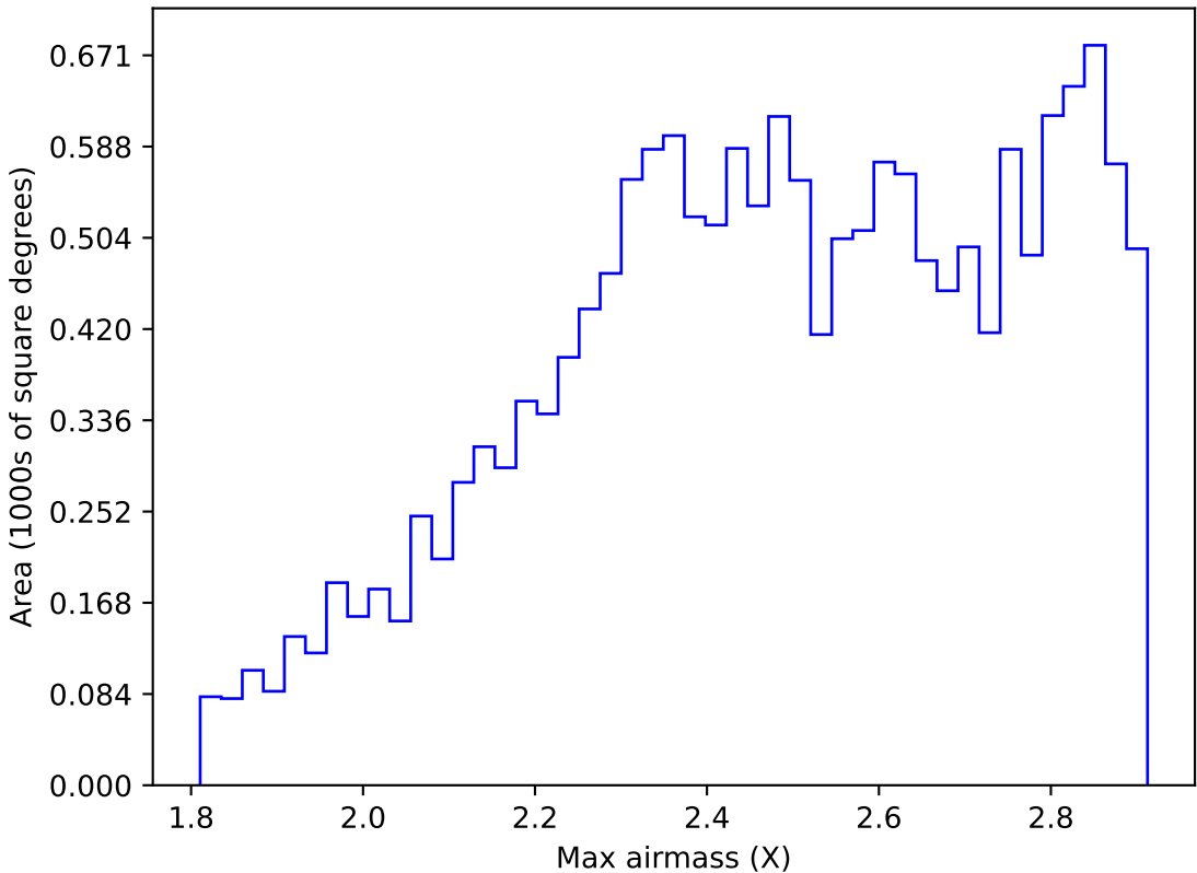
too_elab_r64_d3_ugrizy_v3.4_10yrs WFD z band: Max airmass
