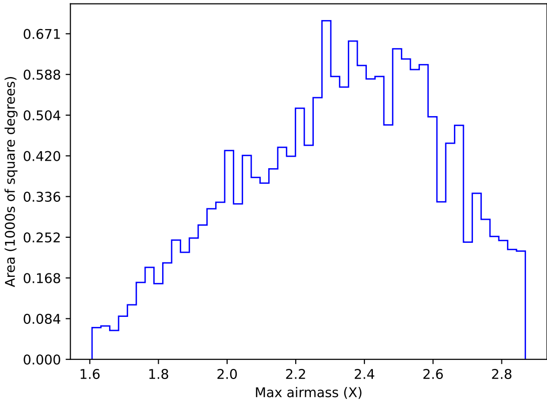
too_elab_r64_d3_ugrizy_v3.4_10yrs WFD y band: Max airmass
