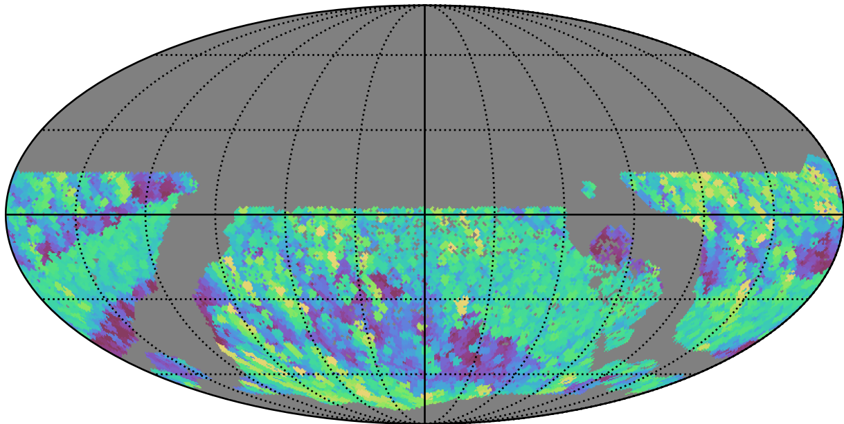
too_elab_r64_d3_ugrizy_v3.4_10yrs WFD r band: Max airmass
