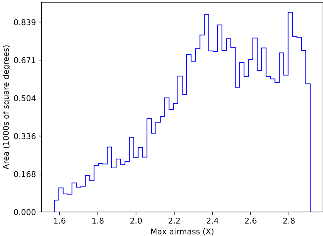
too_elab_r64_d3_ugrizy_v3.4_10yrs All sky z band: Max airmass
