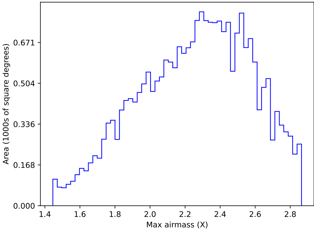
too_elab_r64_d3_ugrizy_v3.4_10yrs All sky y band: Max airmass
