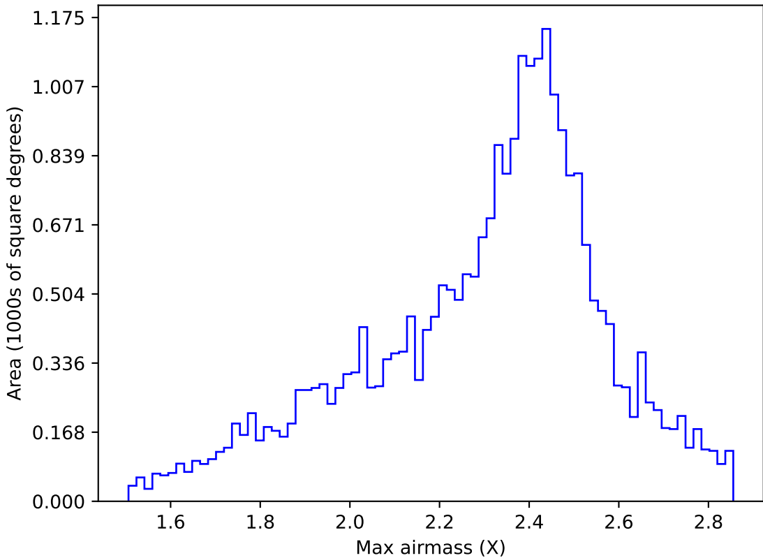
too_elab_r64_d3_ugrizy_v3.4_10yrs All sky r band: Max airmass
