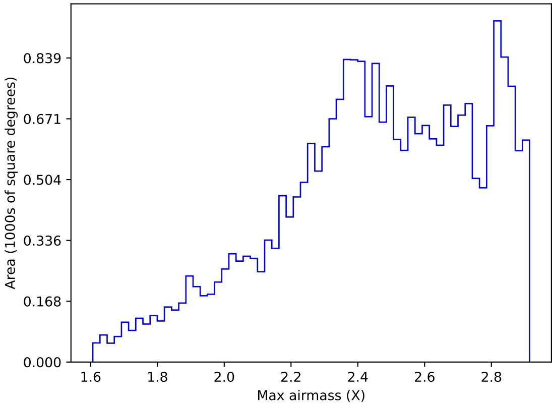
too_elab_r64_d3_ugrizy_v3.4_10yrs All sky i band: Max airmass
