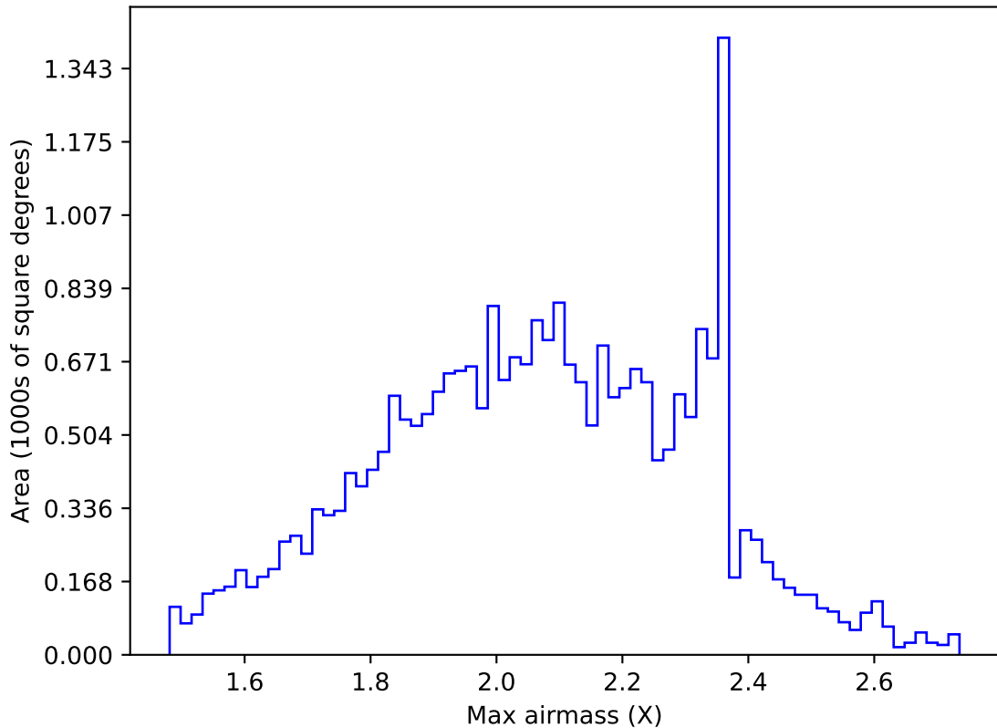
too_elab_r64_d3_ugrizy_v3.4_10yrs All sky g band: Max airmass
