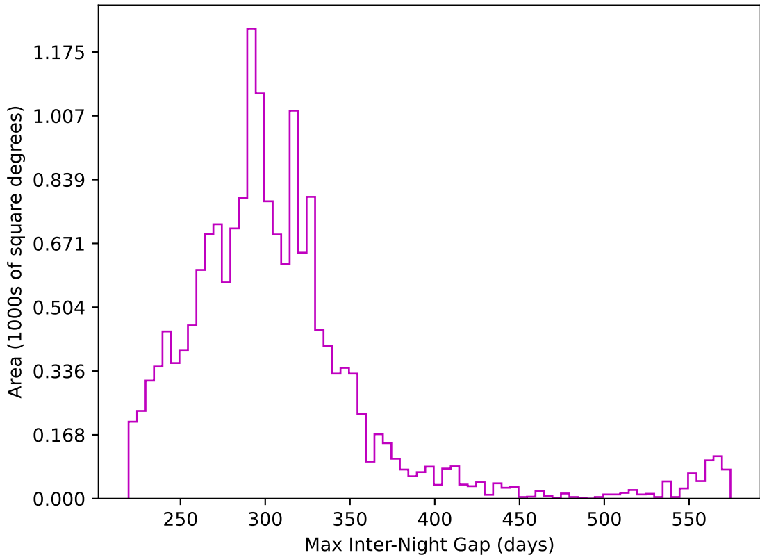
too_elab_r64_d3_ugrizy_v3.4_10yrs WFD z band: Max Inter-Night Gap
