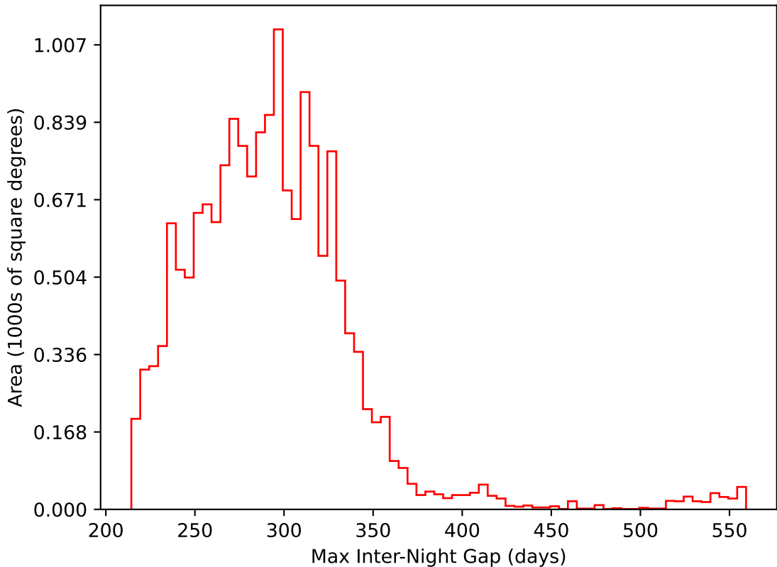
too_elab_r64_d3_ugrizy_v3.4_10yrs WFD i band: Max Inter-Night Gap
