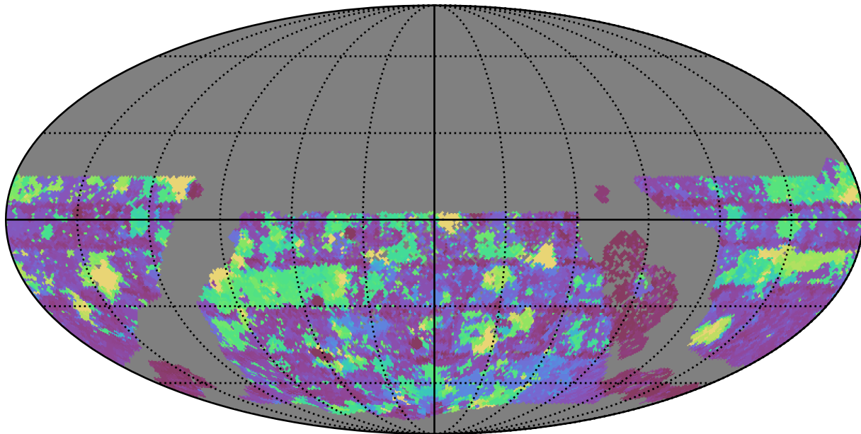
too_elab_r64_d3_ugrizy_v3.4_10yrs WFD g band: Max Inter-Night Gap
