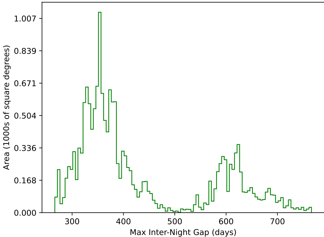
too_elab_r64_d3_ugrizy_v3.4_10yrs WFD g band: Max Inter-Night Gap
