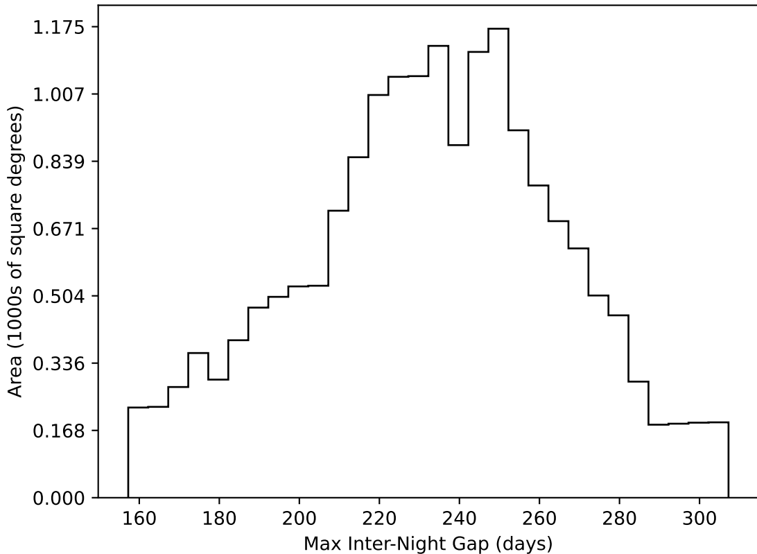
too_elab_r64_d3_ugrizy_v3.4_10yrs WFD all bands: Max Inter-Night Gap
