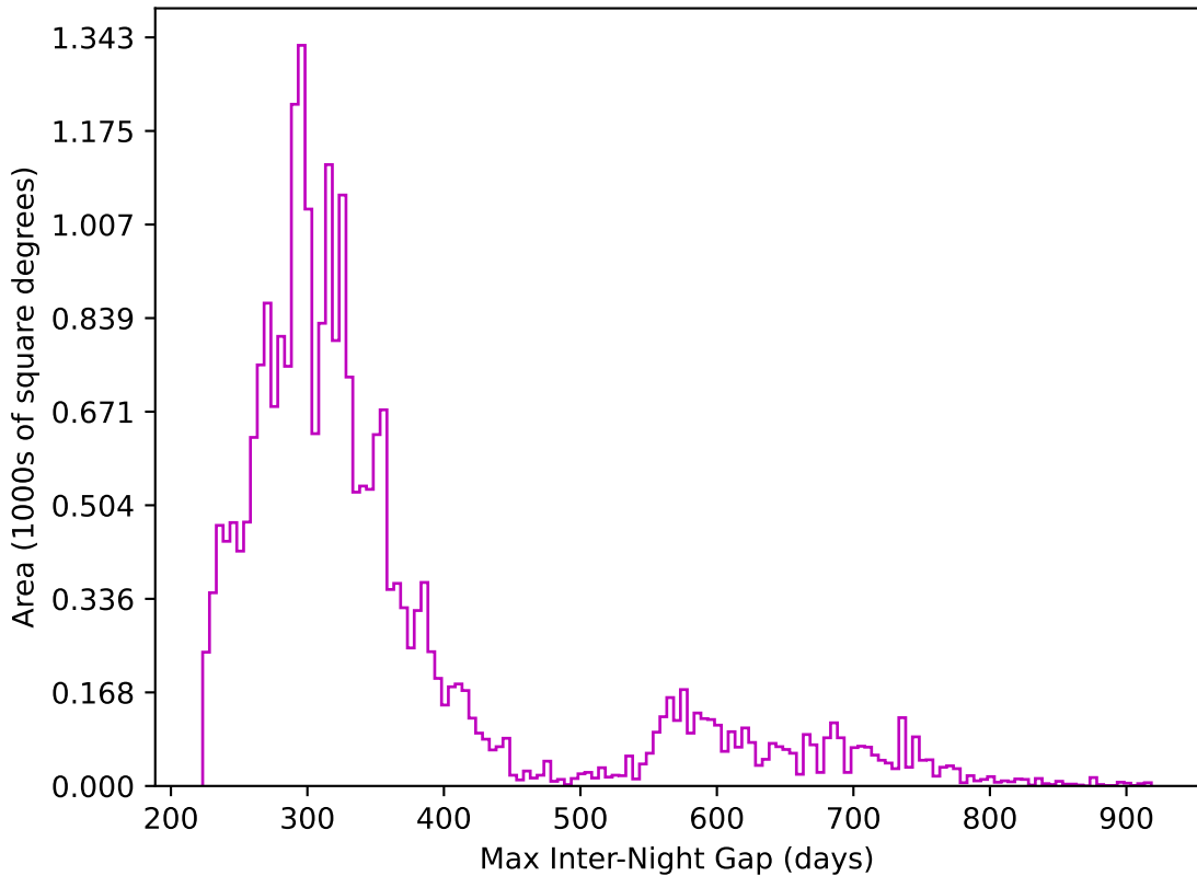
too_elab_r64_d3_ugrizy_v3.4_10yrs All sky z band: Max Inter-Night Gap
