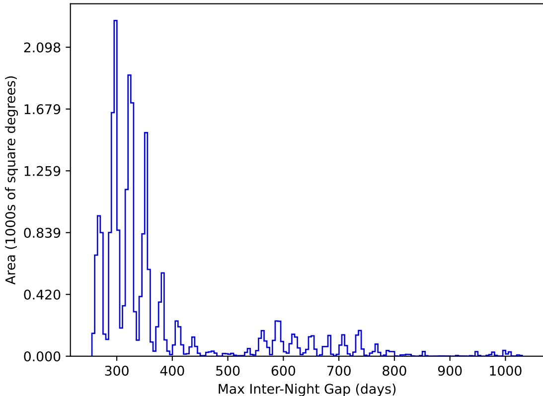
too_elab_r64_d3_ugrizy_v3.4_10yrs All sky y band: Max Inter-Night Gap
