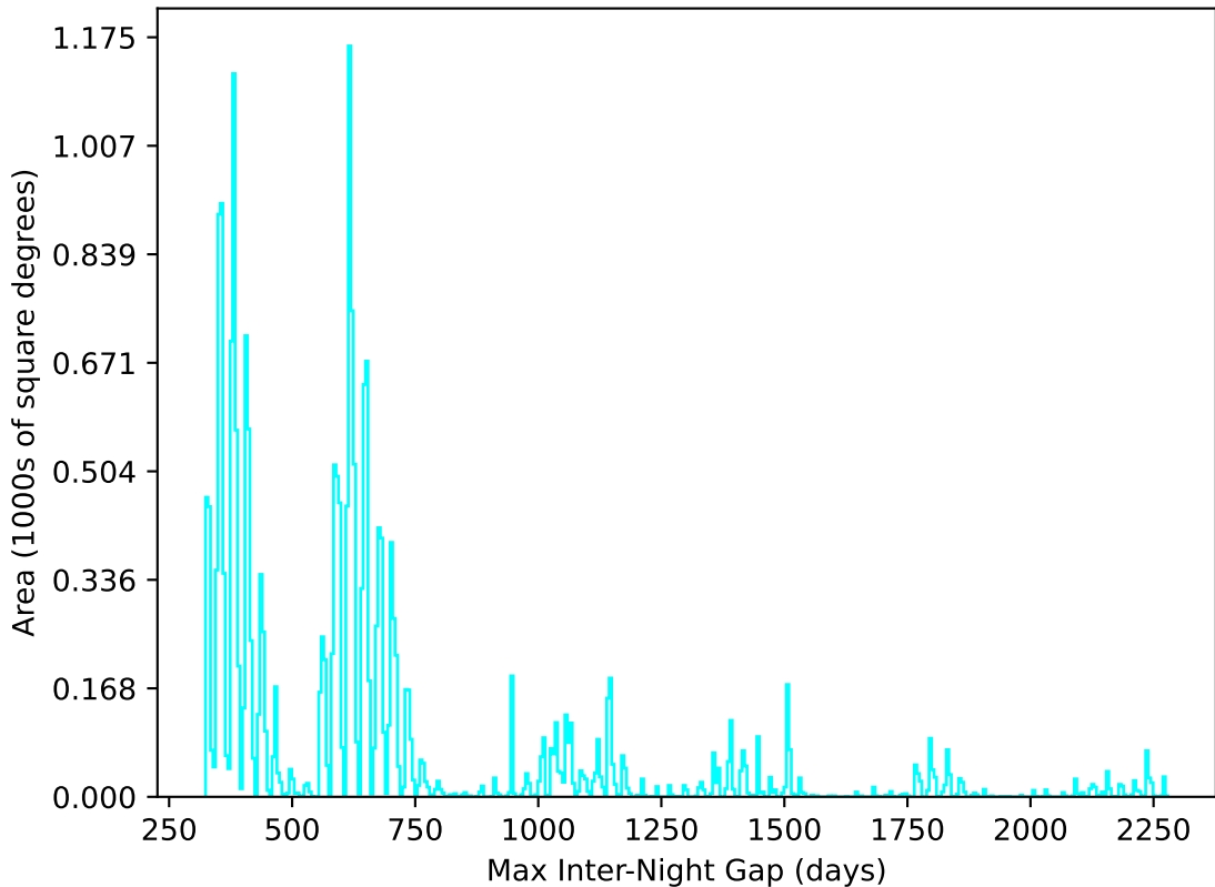
too_elab_r64_d3_ugrizy_v3.4_10yrs All sky u band: Max Inter-Night Gap
