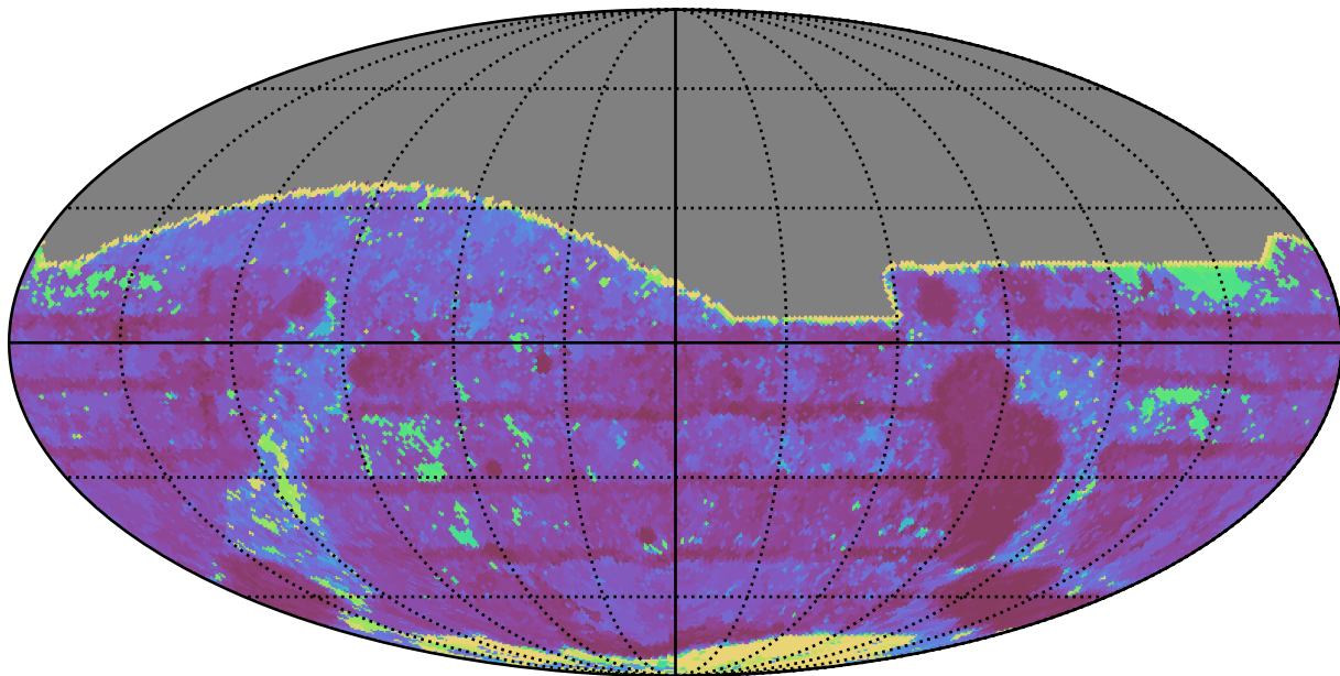
too_elab_r64_d3_ugrizy_v3.4_10yrs All sky r band: Max Inter-Night Gap
