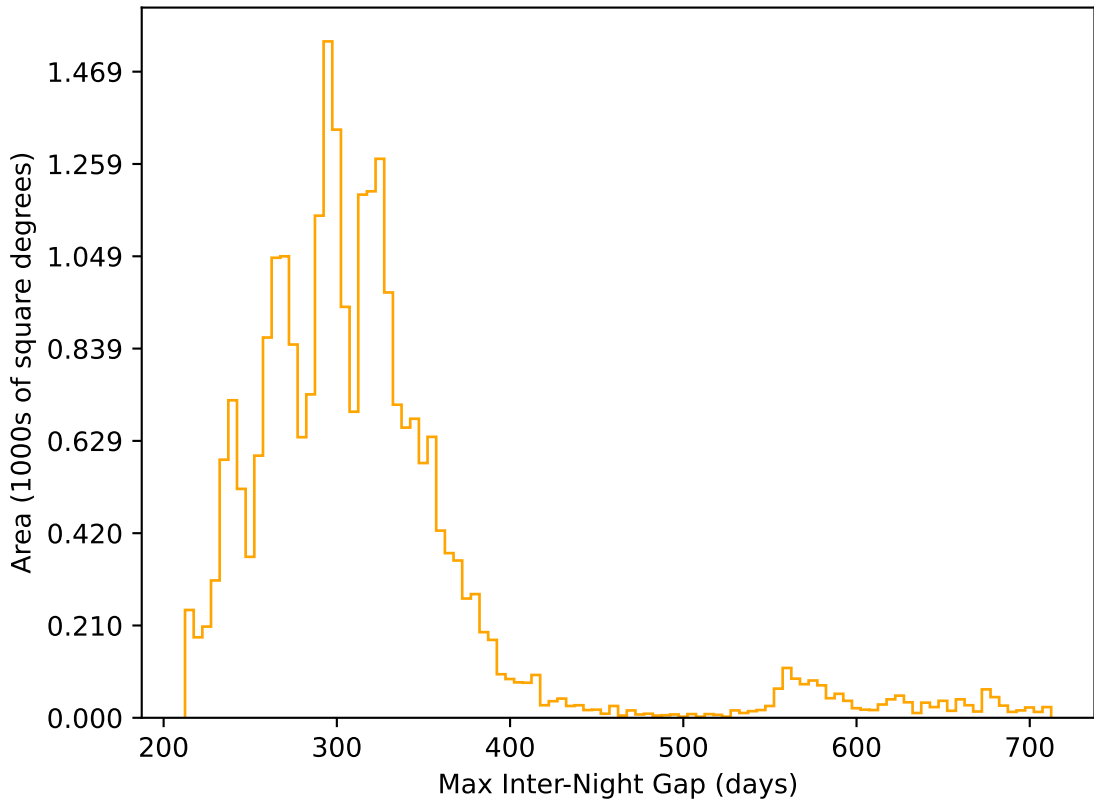
too_elab_r64_d3_ugrizy_v3.4_10yrs All sky r band: Max Inter-Night Gap
