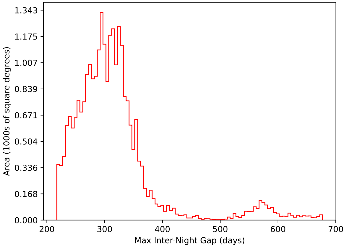
too_elab_r64_d3_ugrizy_v3.4_10yrs All sky i band: Max Inter-Night Gap
