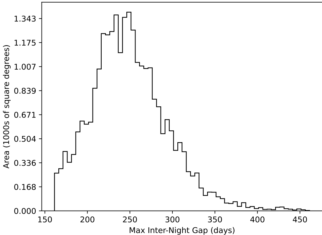
too_elab_r64_d3_ugrizy_v3.4_10yrs All sky all bands: Max Inter-Night Gap
