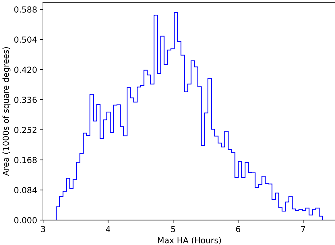
too_elab_r64_d3_ugrizy_v3.4_10yrs WFD z band: Max HA
