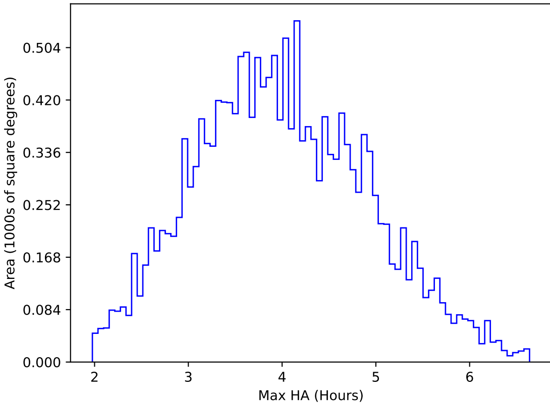
too_elab_r64_d3_ugrizy_v3.4_10yrs WFD u band: Max HA
