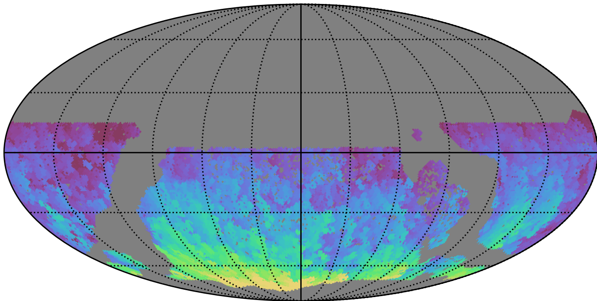
too_elab_r64_d3_ugrizy_v3.4_10yrs WFD r band: Max HA
