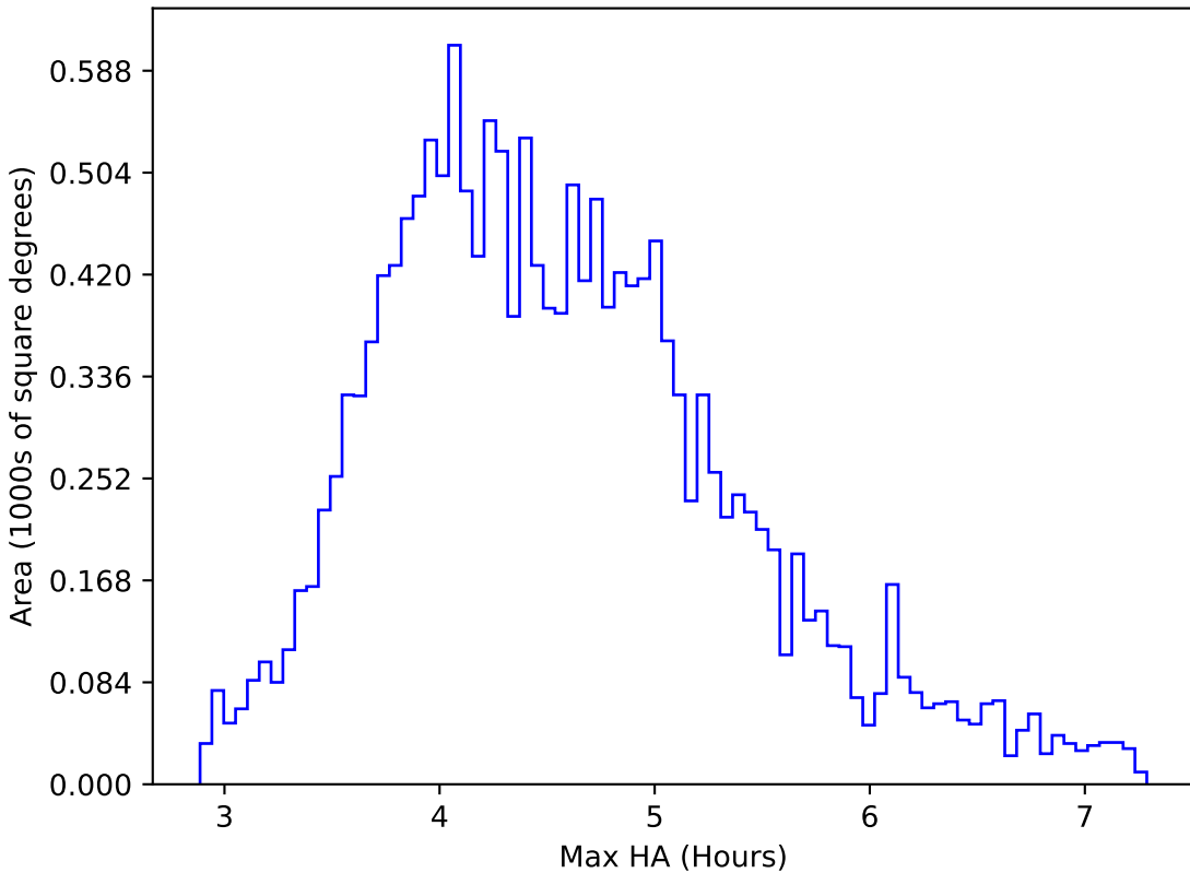
too_elab_r64_d3_ugrizy_v3.4_10yrs WFD r band: Max HA
