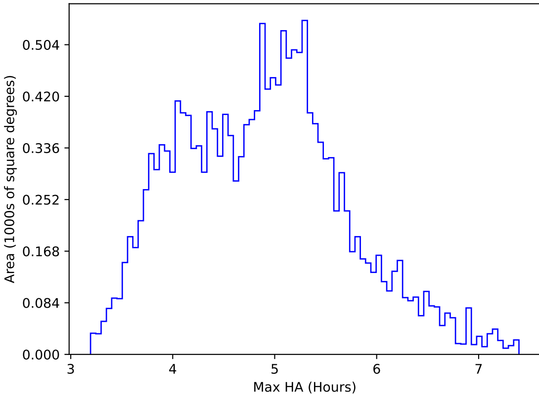
too_elab_r64_d3_ugrizy_v3.4_10yrs WFD i band: Max HA
