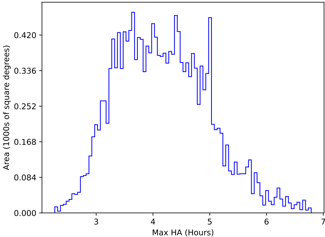
too_elab_r64_d3_ugrizy_v3.4_10yrs WFD g band: Max HA
