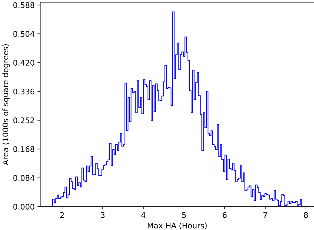
too_elab_r64_d3_ugrizy_v3.4_10yrs All sky z band: Max HA
