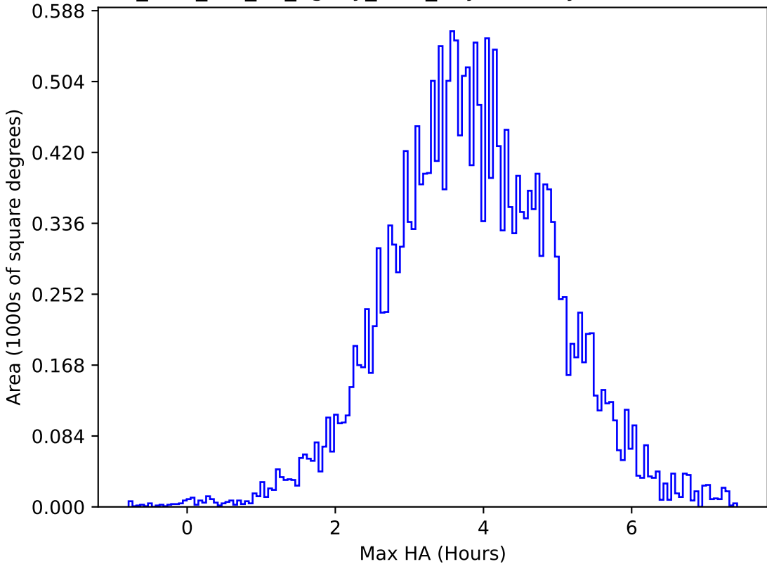
too_elab_r64_d3_ugrizy_v3.4_10yrs All sky u band: Max HA
