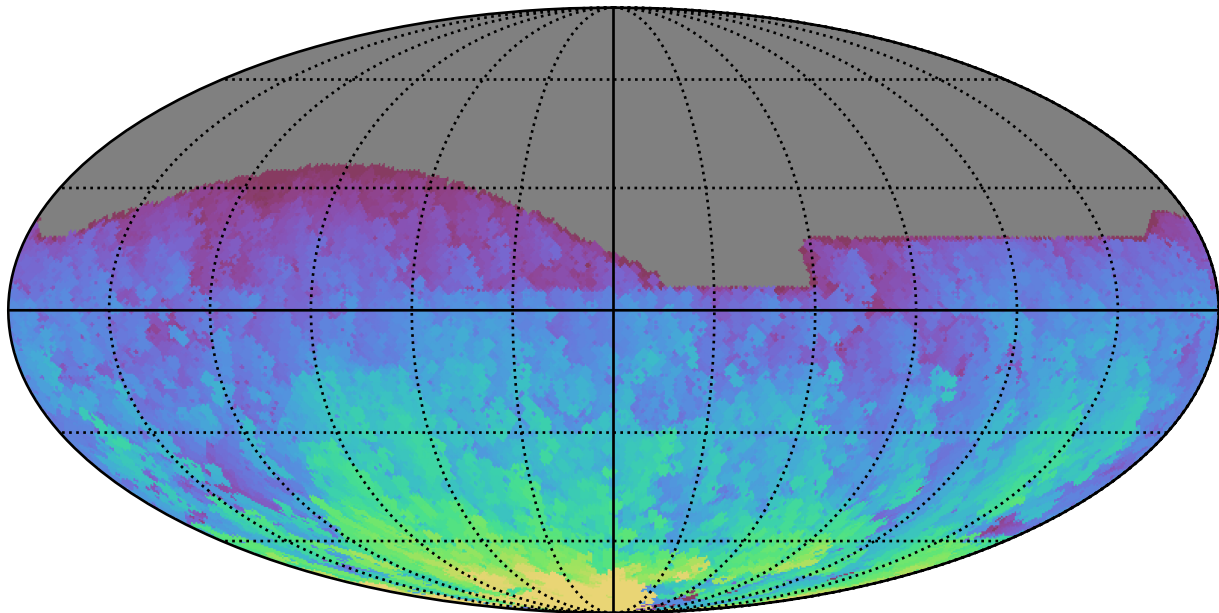
too_elab_r64_d3_ugrizy_v3.4_10yrs All sky r band: Max HA
