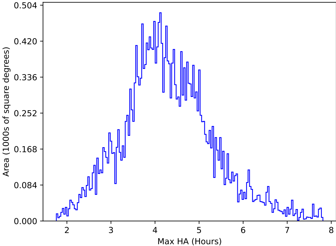
too_elab_r64_d3_ugrizy_v3.4_10yrs All sky r band: Max HA
