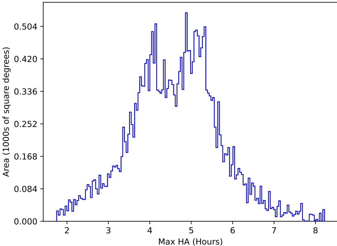
too_elab_r64_d3_ugrizy_v3.4_10yrs All sky i band: Max HA
