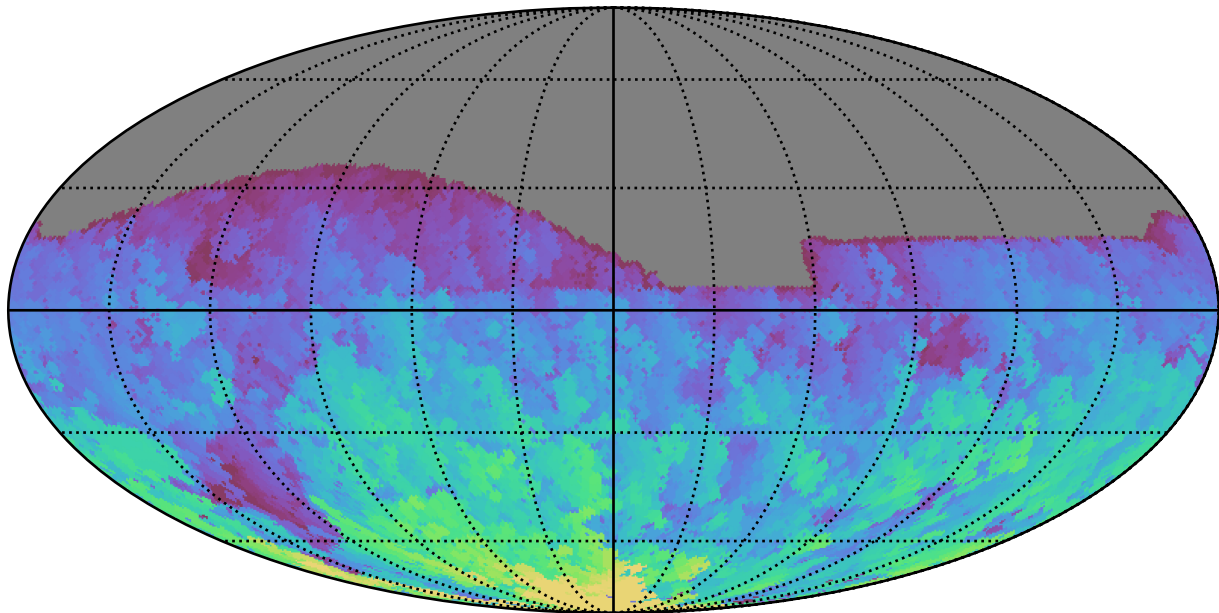
too_elab_r64_d3_ugrizy_v3.4_10yrs All sky g band: Max HA
