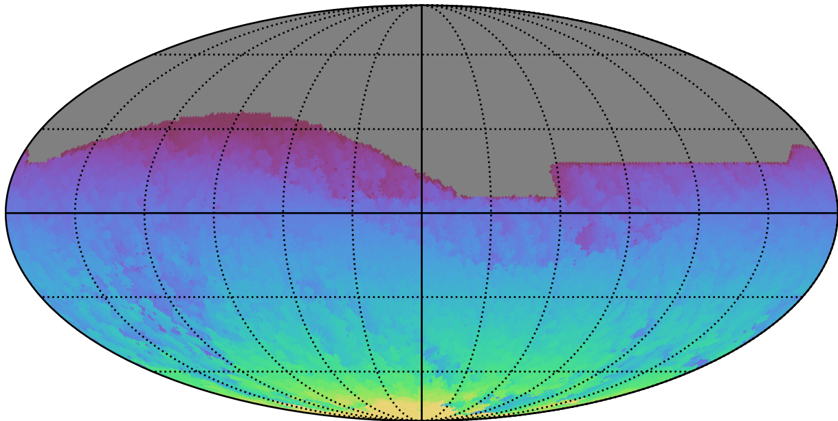
too_elab_r64_d3_ugrizy_v3.4_10yrs All sky all bands: Max HA
