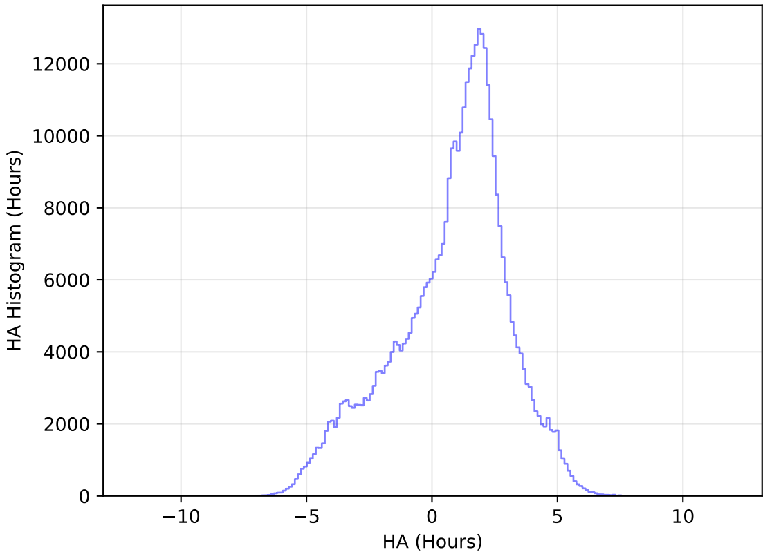
too_elab_r64_d3_ugrizy_v3.4_10yrs WFD z band: HA Histogram
